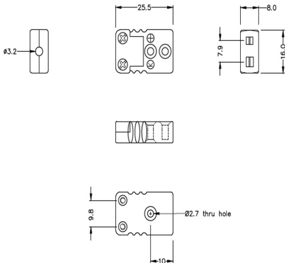
Miniature Hi-Temp Plastic in-line Socket - HTP
